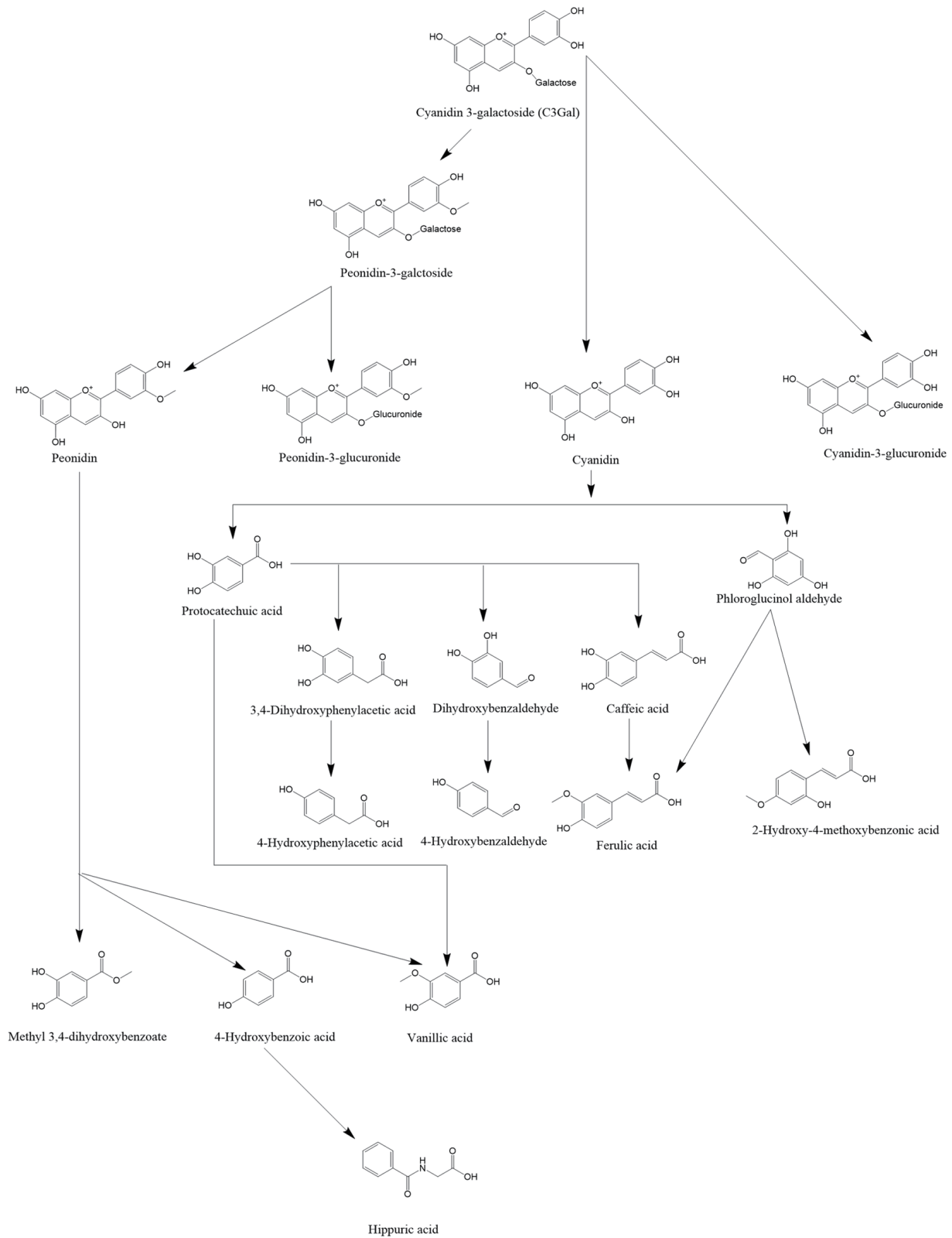
Figure 1. Overview of cyanidin-3-galactoside metabolism, adapted from de Ferrars et al. (2014). Cyanidin-3-galactoside undergoes methylation by the host to form peonidin-3-galactoside, or is hydrolyzed and glucuronidated. Anthocyanins are subsequently hydrolyzed in host tissue or by the gut microbiota into phenolic acids. Phenolic catabolites can undergo enterohepatic circulation and are subjected to further host metabolism prior to excretion.
